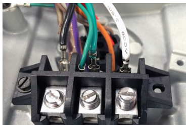
Pre-wired 3-stage terminal block for simplified installation
